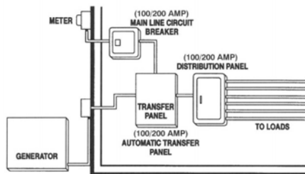
Service entrance installation (USA and Canada) (100/200 A)
